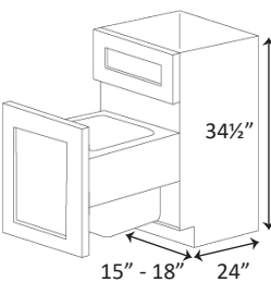
SINGLE/DOUBLE TRASH BIN CABINET 1 DRAWER, 1 PULL OUT DOOR
