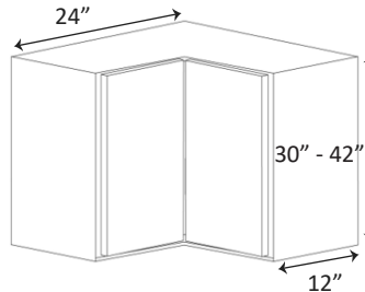
WALL STRAIGHT CORNER CABINET FOLDING DOORS, 3 SHELVES
