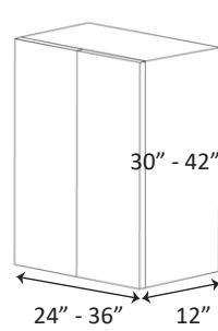
DOUBLE DOOR WALL CABINET 2 DOORS, 3 SHELVES
