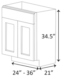
VANITY SINK BASE 2 DOORS
