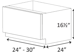
OVEN BASE DRAWER CABINET 1 DRAWER
