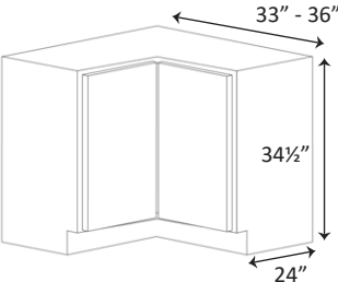
LAZY SUSAN CABINET FOLDING DOORS, 2 TURN TABLES
