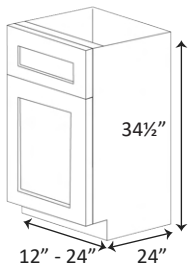
BASE CABINET 1 DRAWER, 1 DOOR, 1 SHELF
