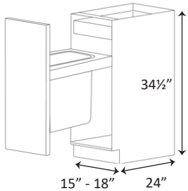
SINGLE/DOUBLE TRASH BIN CABINET 1 DOOR, 1 HIDDEN DRAWER
