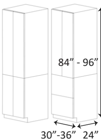
DOUBLE DOOR TALL PANTRY 2 DOORS, 4 SHELVES
