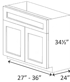
BASE/ SINK BASE CABINET 1 DRAWER, 2 DOORS, 1 SHELF
