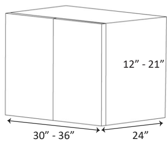
WALL CABINET 2 DOORS
