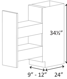
SPICE RACK CABINET 1 DOOR, 2 TIER LEVEL PULL OUT, PRE-ASSEMBLED
